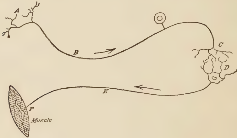
FIG. 1. Two neurones with synapse.
